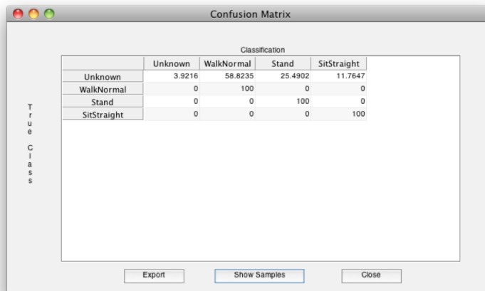
Figure 1.11: WHISFT: classification statistic
