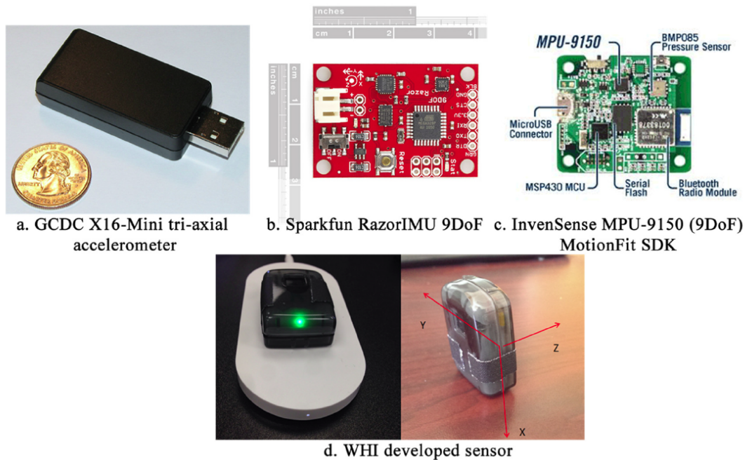
Figure 1.4: Sensors used/developed by Wireless Health Institute (WHI)
