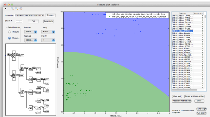
Figure 1.9: WHISFT: decision tree and feature selection
