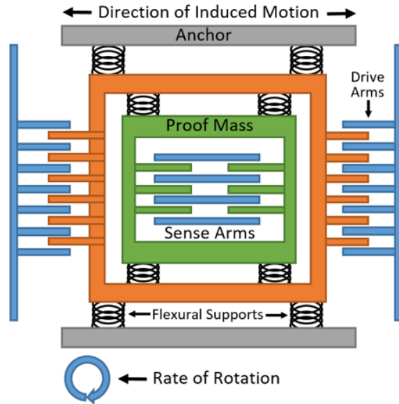
Figure 1.3: Example diagram of a MEMS gyroscope
