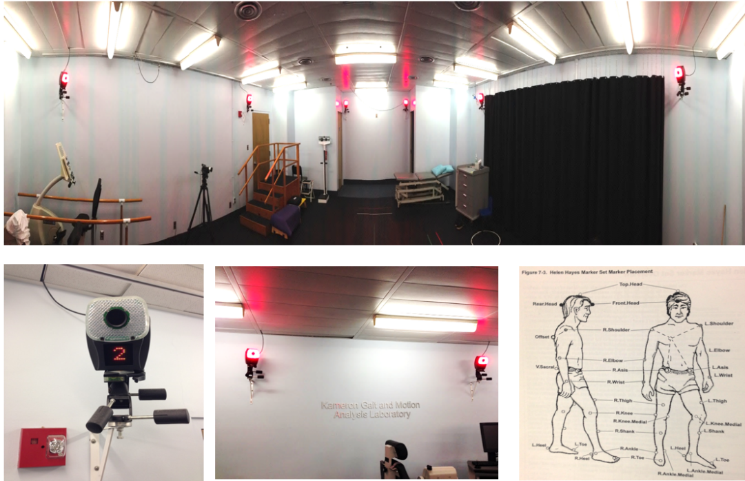
Figure 3.8: Gait and motion analysis lab
